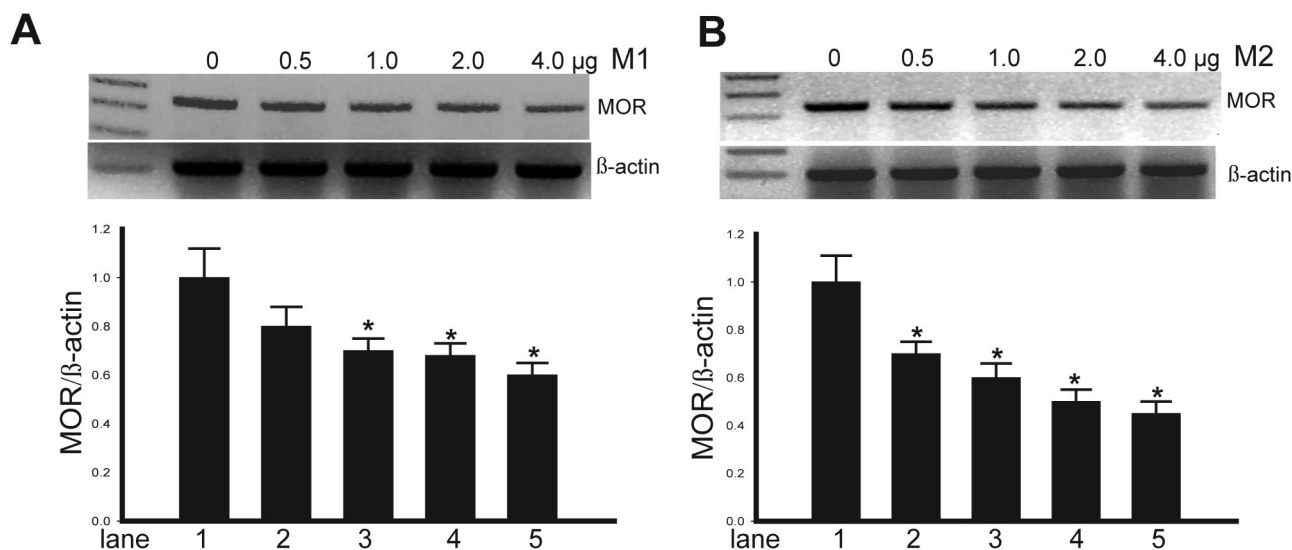
Fig. 8. MOR mRNA expression levels in Sp3 isoform (M1 and M2) cDNA-transfected NMB cells. A, total RNAs from NMB cells transfected with a varying amount of pcDNA-M1/flu plasmid was reverse-transcribed into cDNA that was used as a template for PCR using MOR gene-specific PCR primers and \beta -actin primers as indicated. B, pcDNA-M2/flu was instead of pcDNA-M1/flu. PCR products were electrophoresed on a 2% agarose gel, and the relative densities of MOR mRNA were normalized to \beta -actin. Lane 1, vector DNA only transfected; lane 2, 0.5 \mu g of each plasmid DNA was transfected; lane 3, 1 \mu g of each plasmid DNA was transfected; lane 4, 2 \mu g of each plasmid DNA was transfected; and lane 5, 4 \mu g of each plasmid DNA was transfected. The total amount of DNA transfected was equalized by using vector pcDNA3 DNA. The results of at least three independent transfection experiments performed in triplicate plus S.E.M. are shown. *, p < 0.05 .
