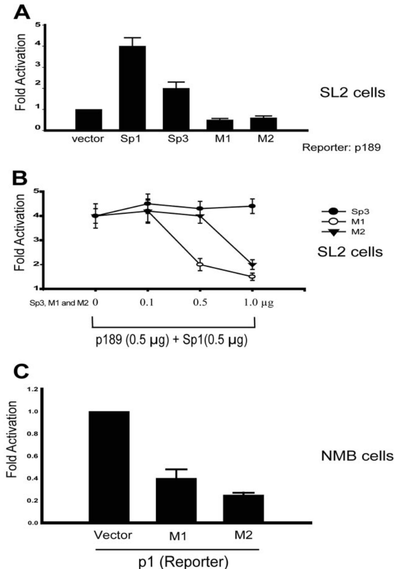
Fig. 7. Effects of Sp1, Sp3, and Sp3 isoforms (M1 and M2) on mMOR promoter in SL2 cells and effects of M1 and M2 on mMOR promoter in NMB cells. A , trans -activation of the mMOR promoter by Sp1 and Sp3 and repression of the mMOR promoter by the Sp3 isoforms (M1 and M2). SL2 cells were cotransfected with 0.5 \mu g of the mMOR promoter construct p189 and 0.5 \mu g of Sp transcription factors (pPacSp1, pPacSp3, pPacM1, and pPacM2). B , effect of Sp3 isoforms (M1 and M2) on the Sp1-mediated trans -activation of mMOR promoter. SL2 cells were cotransfected with 0.5 \mu g of pPacSp1 and different amounts of Sp transcription factors (pPacSp3, pPacM1, and pPacM2) along with 0.5 \mu g of the mMOR promoter construct p189. C , effect of Sp3 isoforms (M1 and M2) on mMOR promoter in NMB cells. NMB cells were cotransfected with 1 \mu g of pcDNA-M1/flu and pcDNA-M2/flu along with 0.5 \mu g of the mMOR promoter construct p1. Cells were harvested 48 h after transfection, lysed, and assayed for luciferase activity and results from at least two representative experiments were averaged. The promoter activity was normalized by protein concentration. Error bars indicate the range of standard errors.
