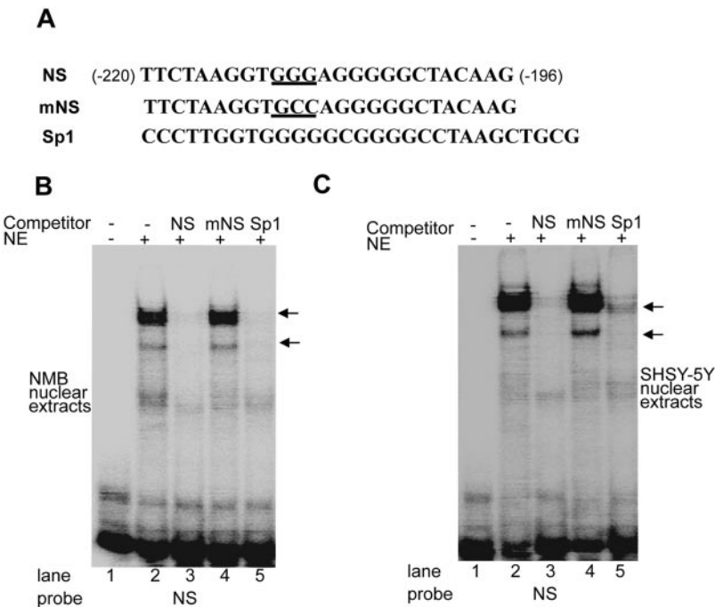
Fig. 4. Binding of nuclear proteins to the negative regulatory element. A , negative regulatory sequence (NS) was used as a probe in EMSA analysis. NS and consensus Sp1 sequence were used as competitors and mNS (Sp3 binding site of NS) was mutated as underlined. EMSA was performed with nuclear extracts (NE) from NMB ( B ) and SHSY-5Y ( C ) cells separately. The major protein/DNA complexes are indicated by arrows. Double-stranded NS was selected as a probe and was ^{32} P labeled. All lanes contained NS probe and 5 \mu g of NE from either NMB or SHSY-5Y cells. Lane 1 is NS probe alone. Lane 2 is a control reaction in the absence of competitor. Lanes 3 to 5 contain 100 M ratio excess of unlabeled NS (lane 3), mNS (lane 4), and consensus Sp1 sequence (lane 5) as specific competitors.
