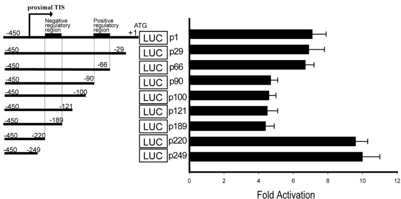
Fig. 1. 3'-Deletion analysis of proximal promoter activity of \mu opioid receptor gene. A schematic diagram representing the proximal promoter region of the mouse MOR gene from nucleotide -450 to +1. The translation start site (ATG) is designated as +1. Fragments of various lengths of the promoter region were inserted into the promoterless luciferase vector, pGL3-basic (Promega). The numbers on the right of each construct refer to the number of the nucleotide at the 3' end of each inserted promoter fragment. The numbers on the left of each construct refer to the number of the nucleotide at the 5' end of each construct, which is -450 bp. Transient transfections and luciferase assays of various constructs were performed in NMB cells as described under Materials and Methods . The proximal activity of each construct was expressed as n -fold activation of pGL3-basic promoter activity. The histograms represent the mean values of fold activation from three independent transfection experiments with two different plasmid preparations. Error bars indicate the range of standard errors. TIS, transcription initiation site.
