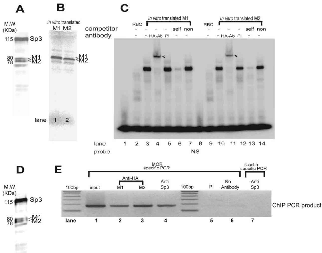
Fig. 6. Supershift assay of in vitro-translated HA-tagged Sp3 isoforms (M1 and M2) using the anti-HA antibody and ChIP assay using Sp3 and HA antibodies. A, Western blot analysis was carried out with nuclear extracts from NMB cells and anti-Sp3 antibody. Three different isoforms of Sp3 with different molecular masses are indicated. M.W. stands for molecular mass in kilodaltons. B, in vitro-translated M1 and M2 proteins were radiolabeled with [ 35 S]methionine using Promega's in vitro translation kit. C, EMSAs were performed as indicated under Materials and Methods . Lanes 2 and 9 are reticulocyte (RBC) EMSA reactions without antibody. Lanes 3 and 10 are the control EMSA reactions without antibody. The supershift band is indicated by <. Lanes 4 and 11 are the EMSA reactions with the HA antibody. Lanes 5 and 12 are reactions with PI serum. Lanes 6 and 13 are self-competitor controls without antibody. All lanes contained 5 \mu l of in vitro-translated M1 and M2 products from a 50- \mu l reaction volume (Promega's in vitro translation kit). In vitro-translated M1 and M2 proteins were incubated with the monoclonal HA antibody, PI serum, or self-competitor as indicated. D, Western blot analysis was carried out with nuclear extracts from NS20Y cells and anti-Sp3 antibody. Three different isoforms of Sp3 with different molecular masses are indicated. M.W. stands for molecular mass in kilodaltons. E, chromatin immunoprecipitation analysis of Sp3 isoforms M1 and M2 binding interaction at MOR promoter. ChIP assay was performed using a Sp3 and HA antibody in NS20Y cells. Immunoprecipitated DNA was analyzed by PCR using primers that amplified a 196-bp region of the MOR promoter, which encompasses a negative regulatory sequence. Lane 1, input; lanes 2 and lane 3, 10 \mu g of HA antibody; lanes 4 and 7, 10 \mu g of Sp3 antibody; lane 5, PI serum; lane 6, no antibody; and lane 7, a negative control of PCR for Sp3 immunoprecipitation using specific primers for mouse \beta -actin gene.
